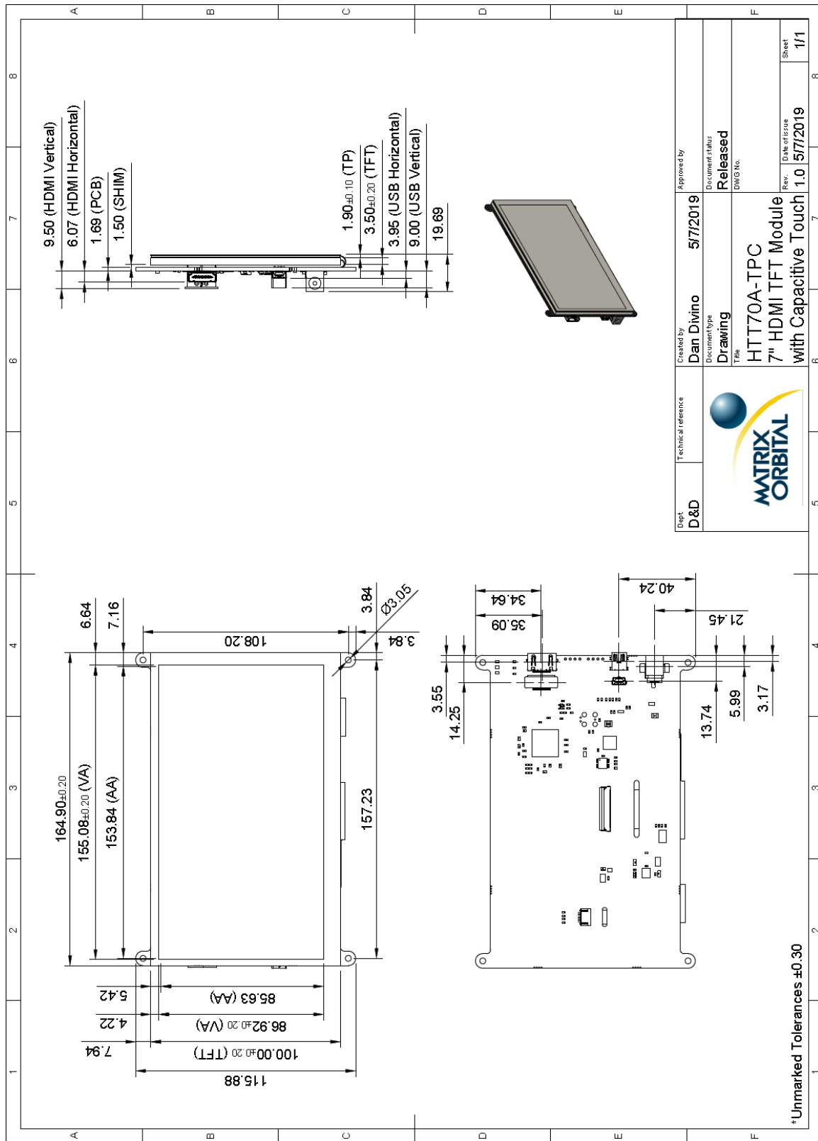
Figure 11: HTT70A-TPC Dimensional Drawing
