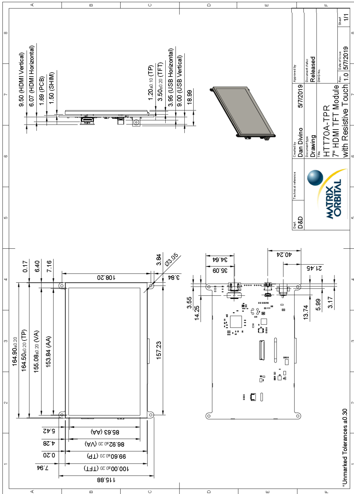
Figure 12: HTT70A-TPR Dimensional Drawing
